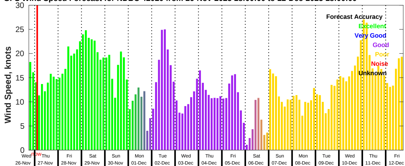
GFS Wind Speed Forecast for NDBC 42020 from 26-Nov-2025 18:00:00 to 12-Dec-2025 18:00:00
