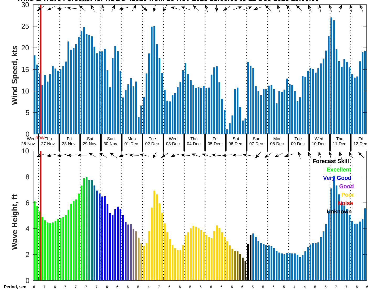
Wind & Wave Forecast for NDBC 42020 from 26-Nov-2025 18:00:00 to 12-Dec-2025 18:00:00
