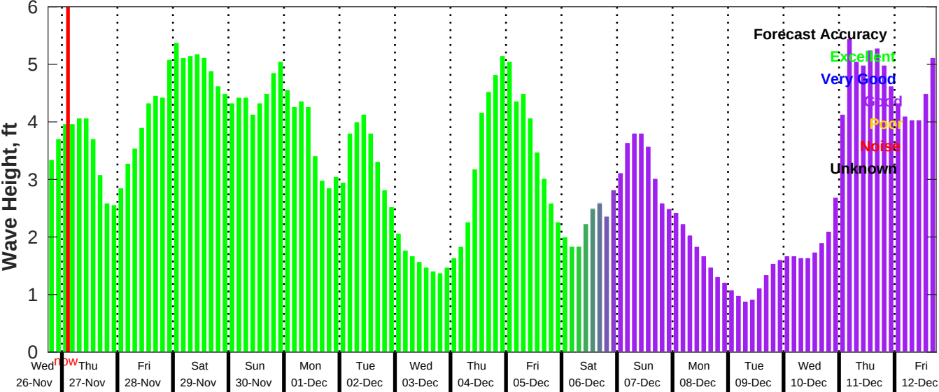
GFS Wave Forecast for NDBC 42035 from 26-Nov-2025 18:00:00 to 12-Dec-2025 18:00:00
