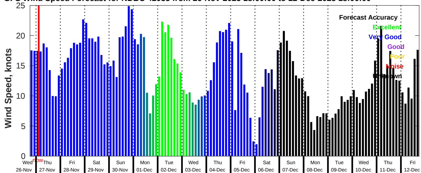
GFS Wind Speed Forecast for NDBC 42035 from 26-Nov-2025 18:00:00 to 12-Dec-2025 18:00:00
