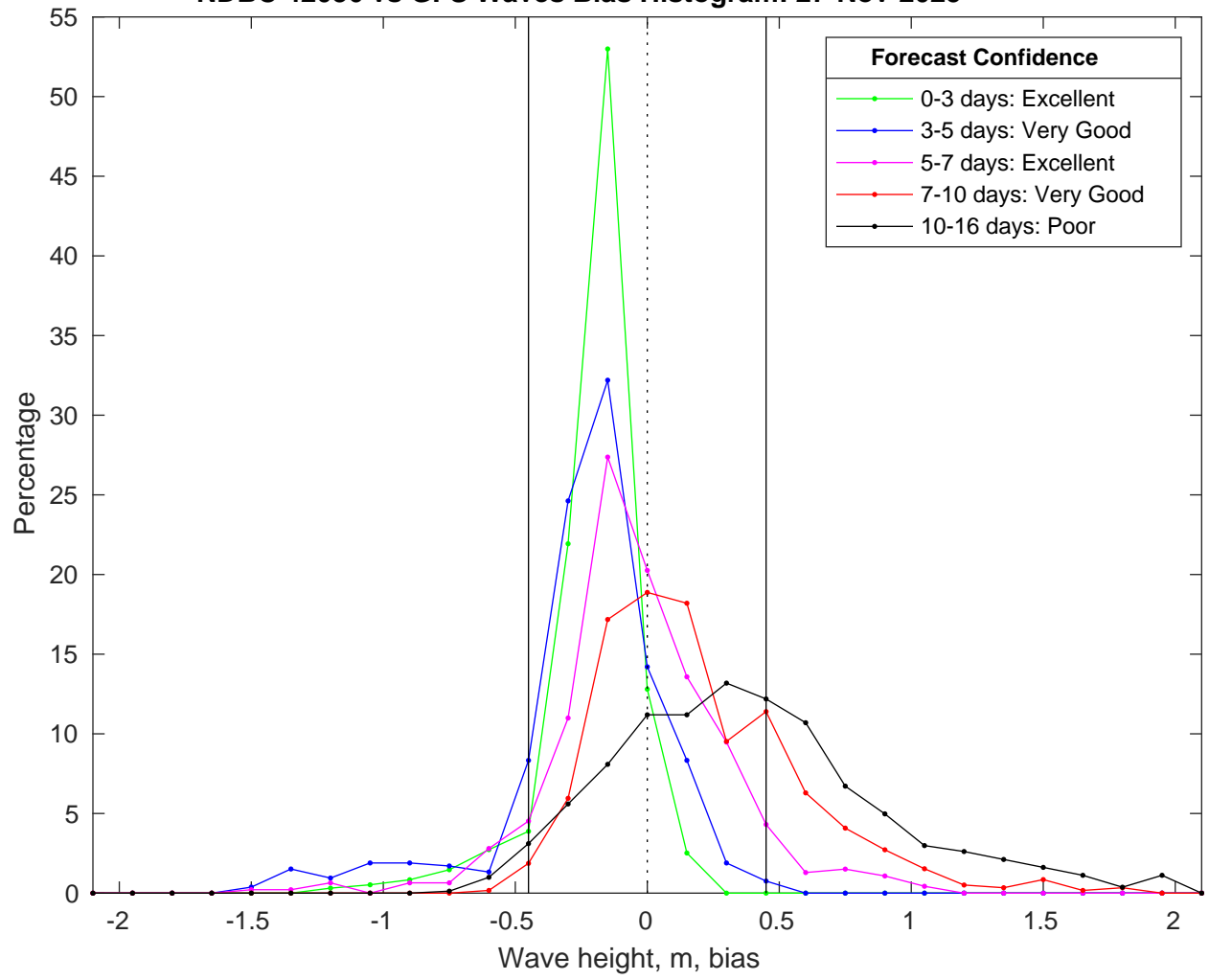
NDBC 42036 vs GFS Waves Bias Histogram: 27-Nov-2025
