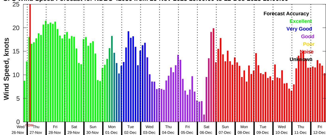
GFS Wind Speed Forecast for NDBC 42036 from 26-Nov-2025 19:00:00 to 12-Dec-2025 19:00:00
