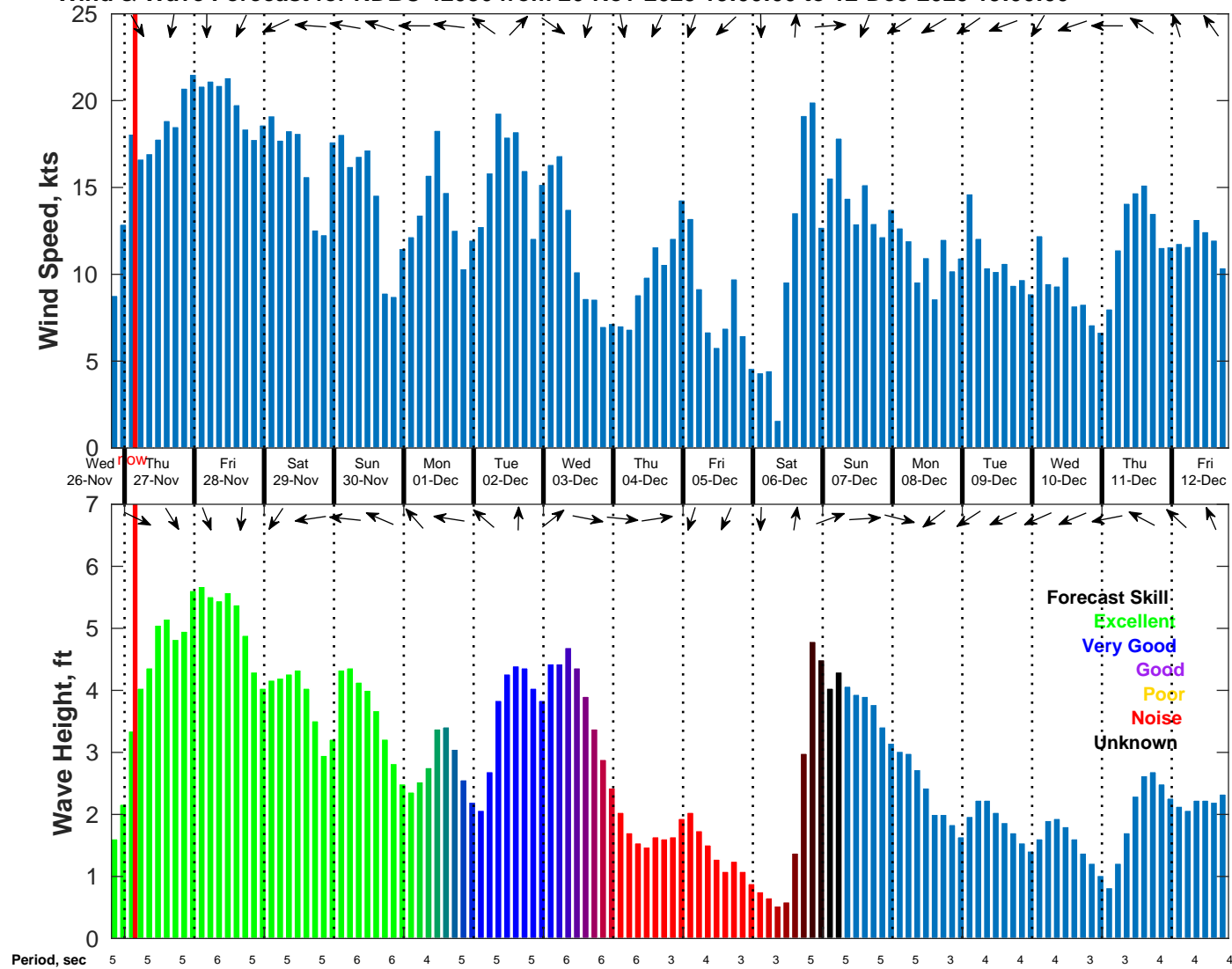
Wind & Wave Forecast for NDBC 42036 from 26-Nov-2025 19:00:00 to 12-Dec-2025 19:00:00
