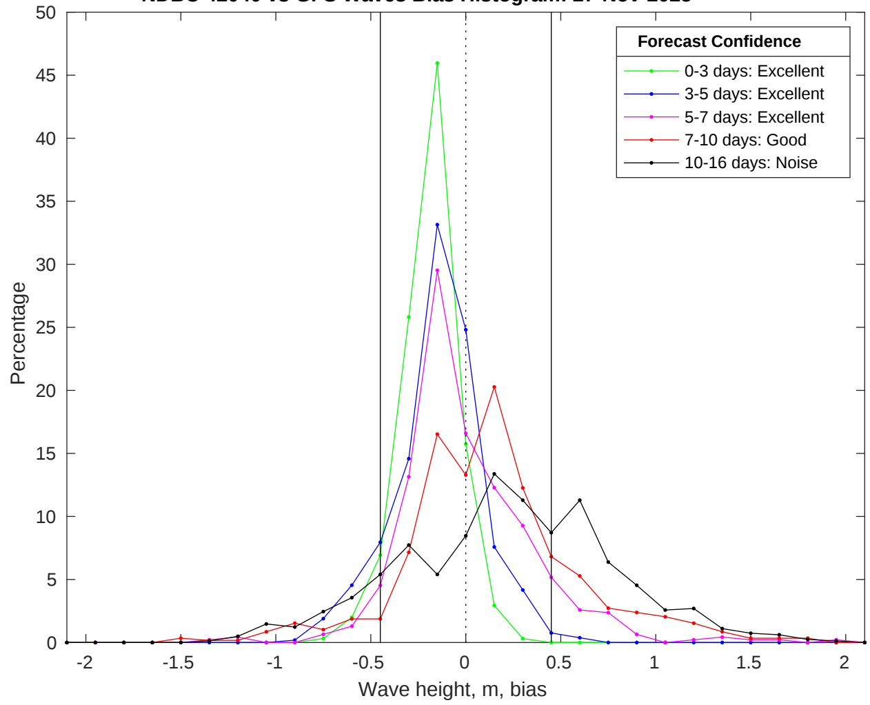
NDBC 42040 vs GFS Waves Bias Histogram: 27-Nov-2025
