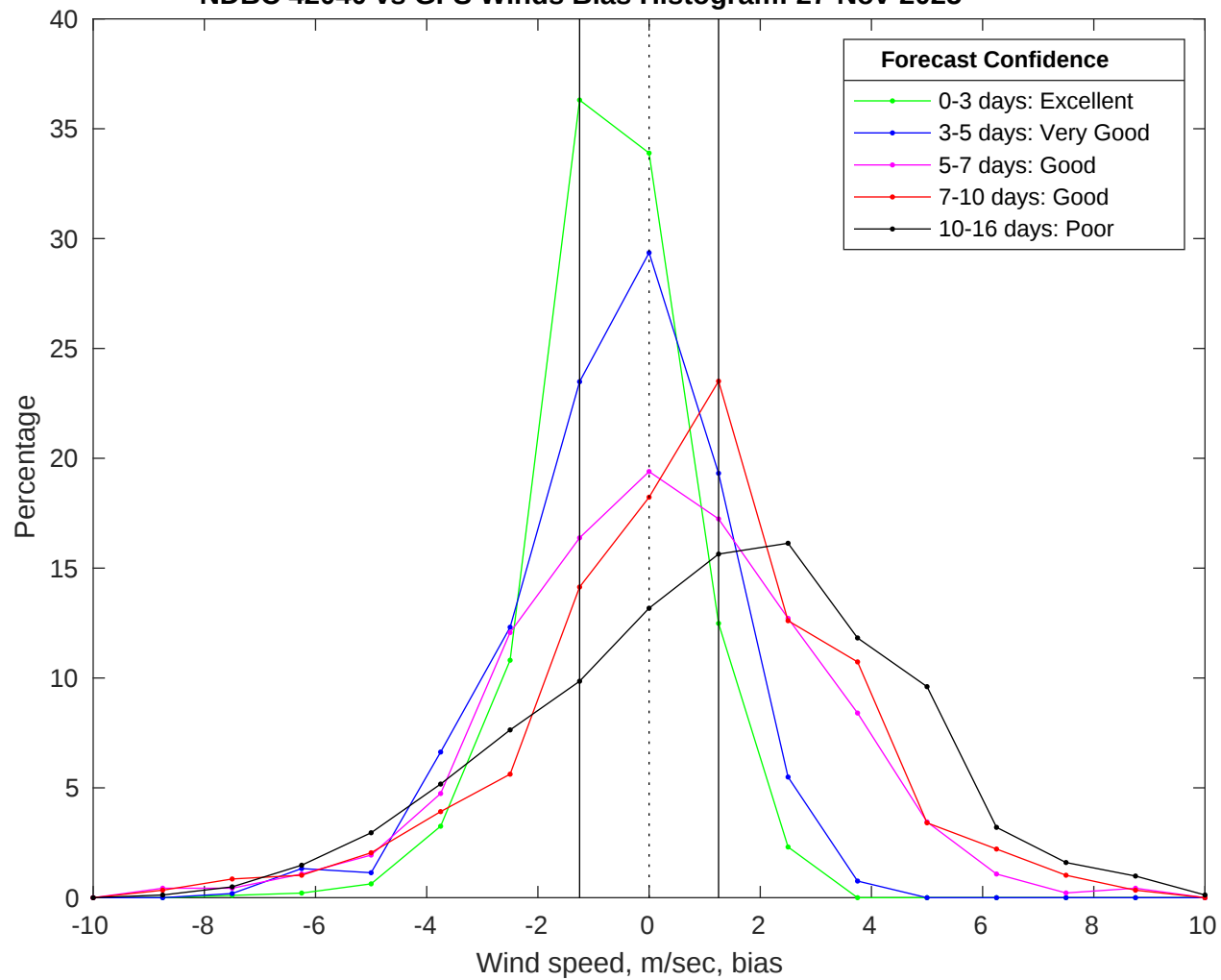
NDBC 42040 vs GFS Winds Bias Histogram: 27-Nov-2025
