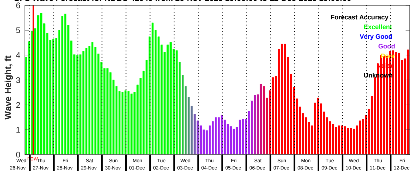
GFS Wave Forecast for NDBC 42040 from 26-Nov-2025 19:00:00 to 12-Dec-2025 19:00:00
