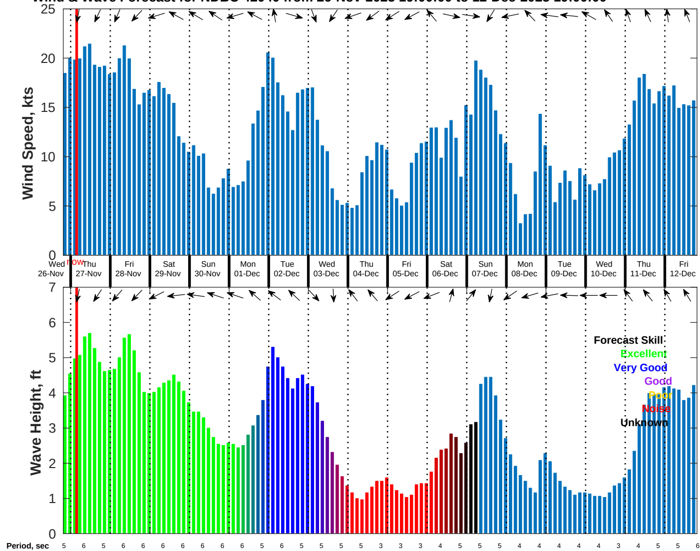
Wind & Wave Forecast for NDBC 42040 from 26-Nov-2025 19:00:00 to 12-Dec-2025 19:00:00
