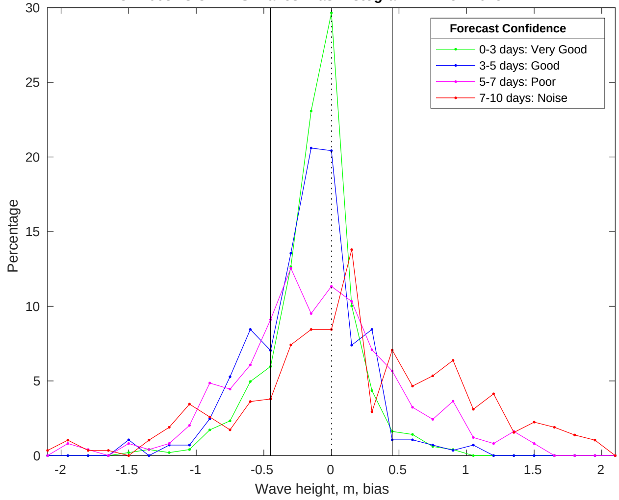
NDBC 44008 vs CMEMS Waves Bias Histogram: 27-Nov-2025
