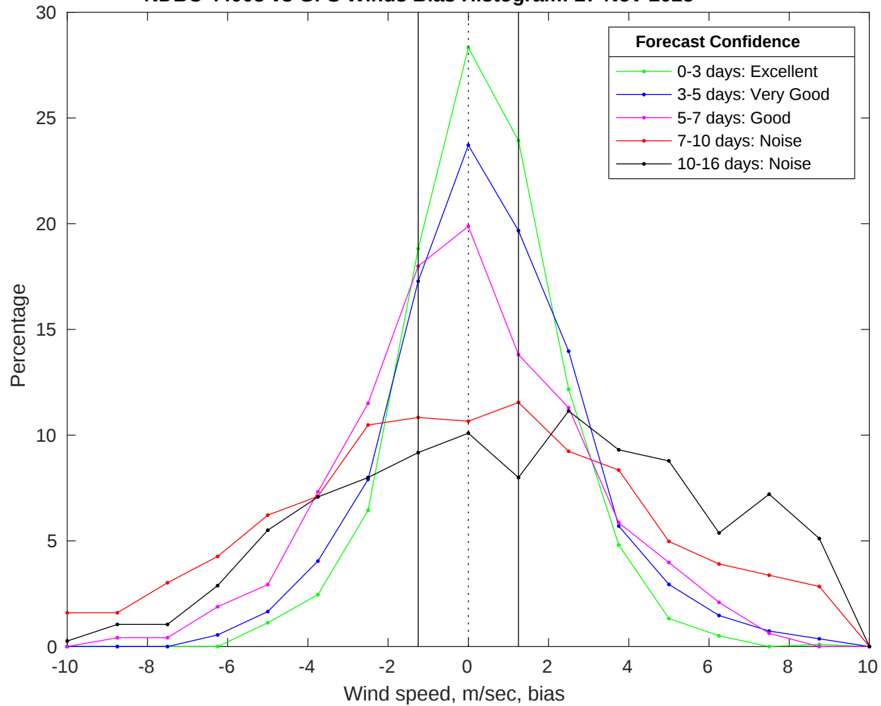
NDBC 44008 vs GFS Winds Bias Histogram: 27-Nov-2025
