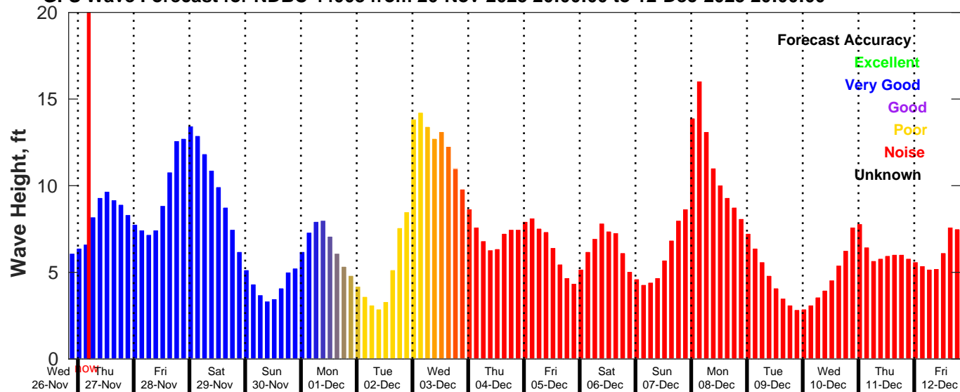
GFS Wave Forecast for NDBC 44008 from 26-Nov-2025 20:00:00 to 12-Dec-2025 20:00:00
