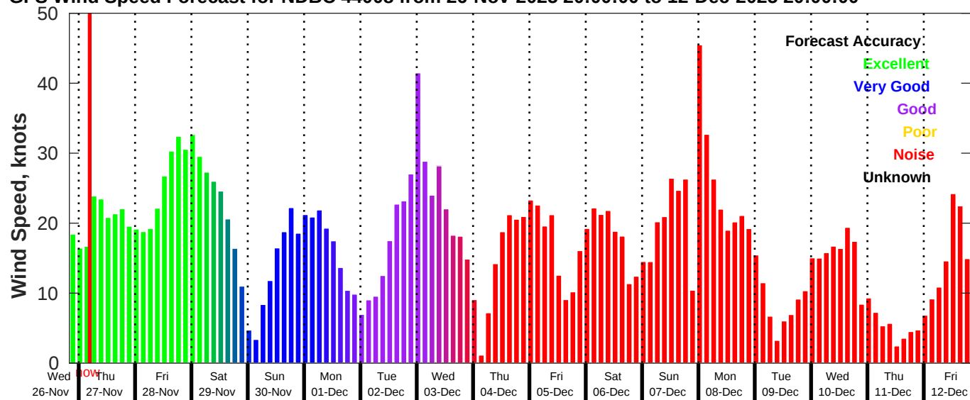
GFS Wind Speed Forecast for NDBC 44008 from 26-Nov-2025 20:00:00 to 12-Dec-2025 20:00:00
