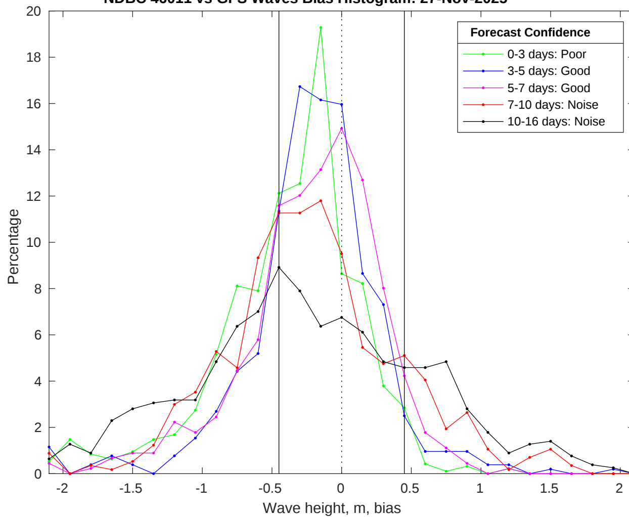
NDBC 46011 vs GFS Waves Bias Histogram: 27-Nov-2025
