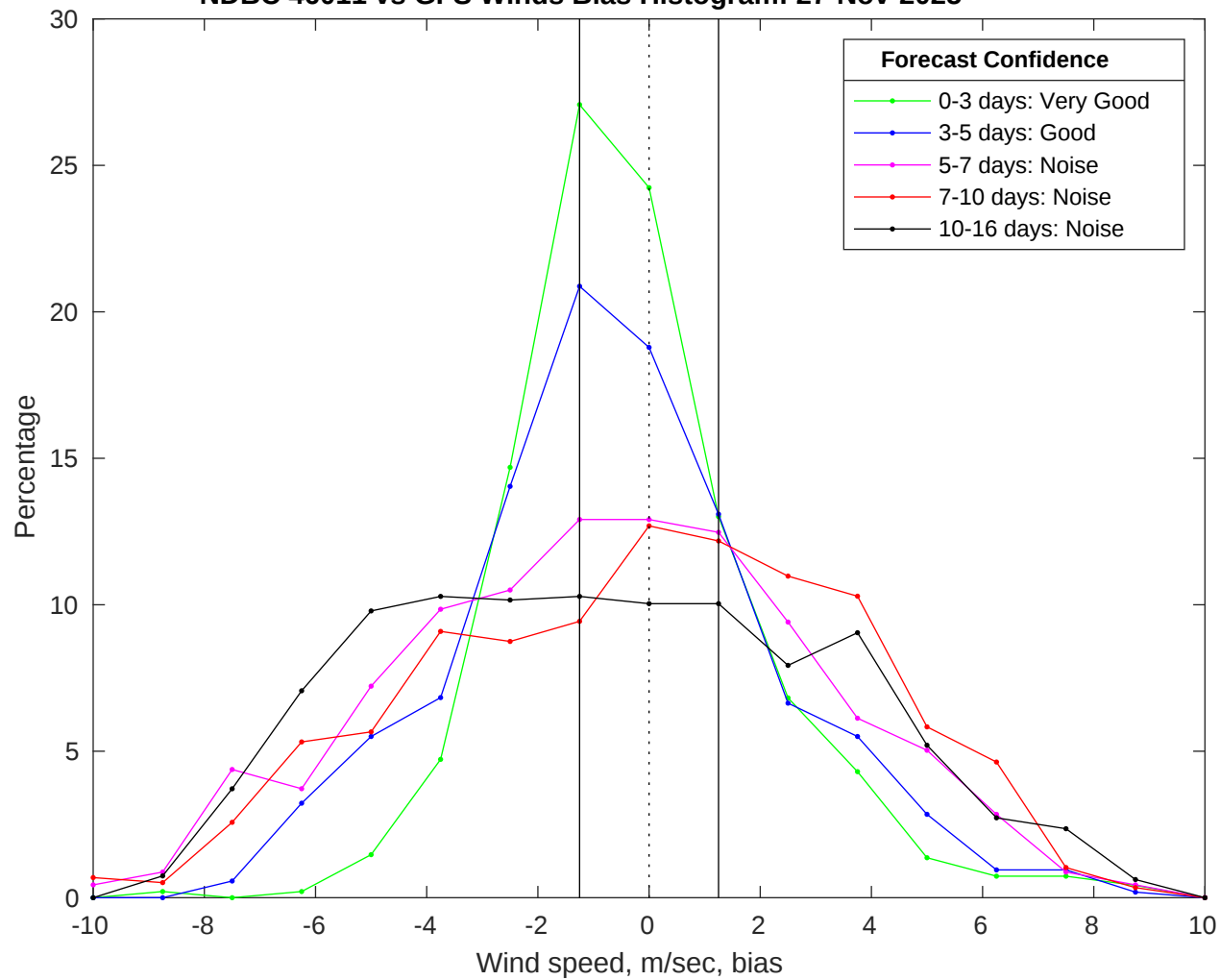
NDBC 46011 vs GFS Winds Bias Histogram: 27-Nov-2025
