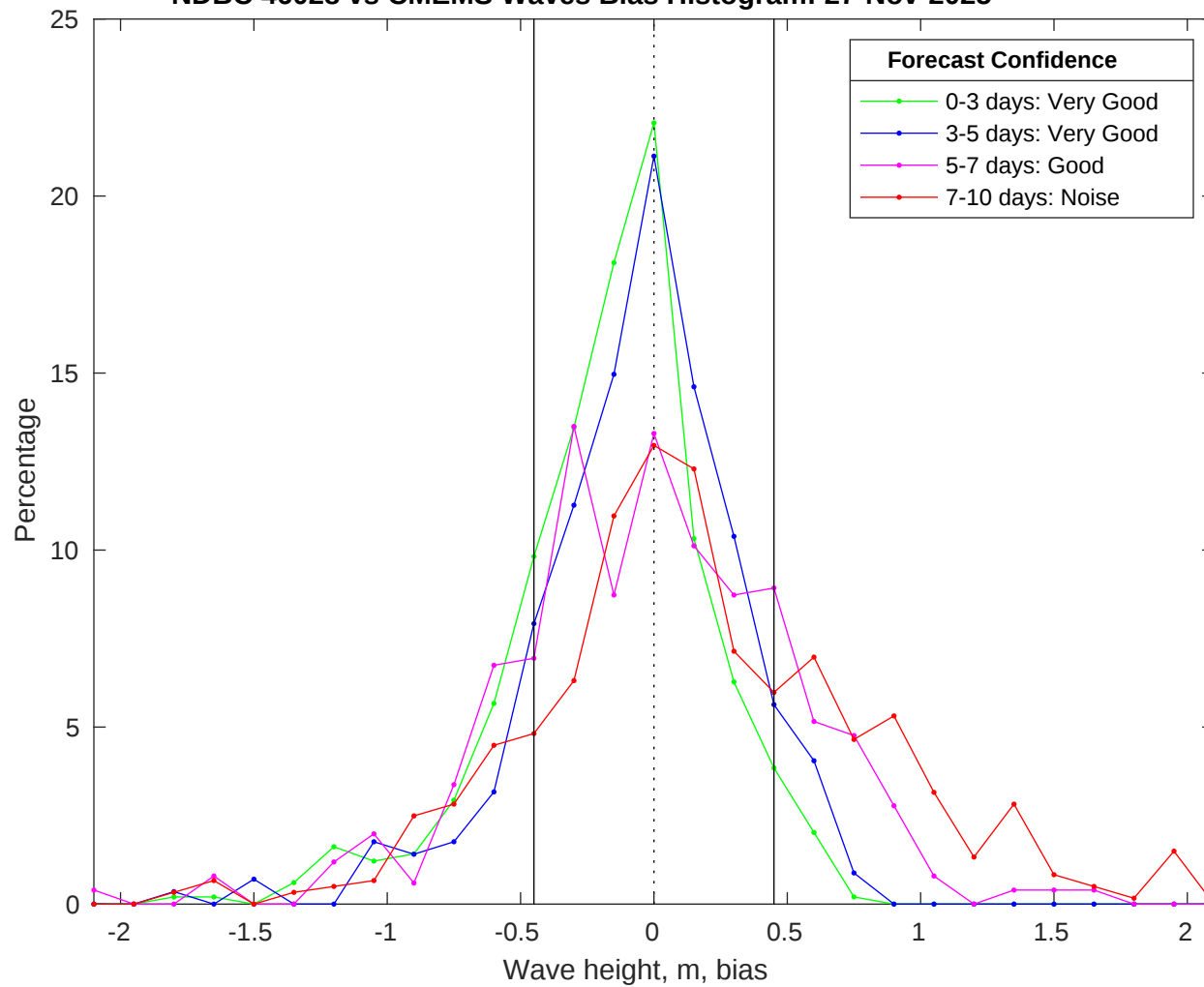
NDBC 46028 vs CMEMS Waves Bias Histogram: 27-Nov-2025
