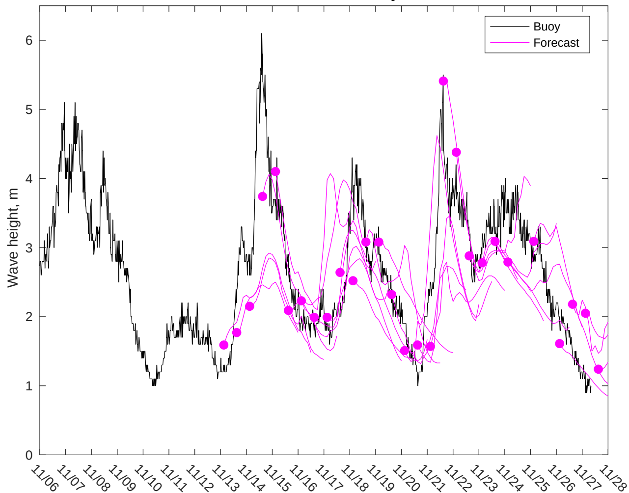
NDBC 46028 vs GFS Waves: 7 to 10 day forecast
