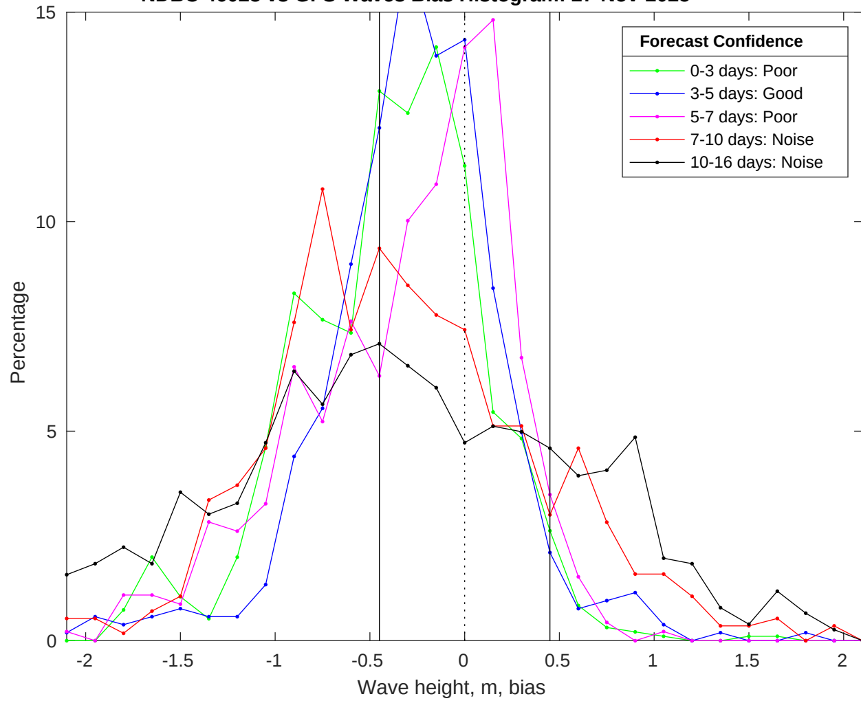
NDBC 46028 vs GFS Waves Bias Histogram: 27-Nov-2025
