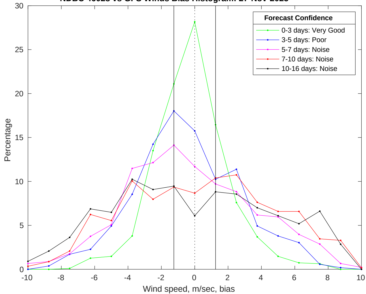
NDBC 46028 vs GFS Winds Bias Histogram: 27-Nov-2025
