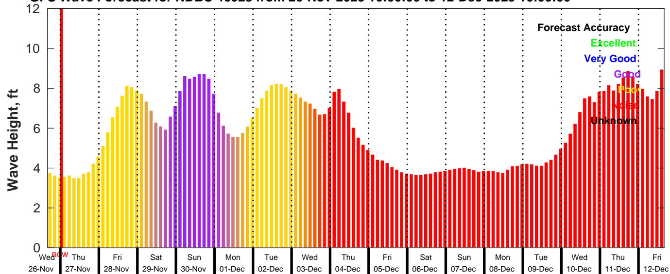
GFS Wave Forecast for NDBC 46028 from 26-Nov-2025 16:00:00 to 12-Dec-2025 16:00:00
