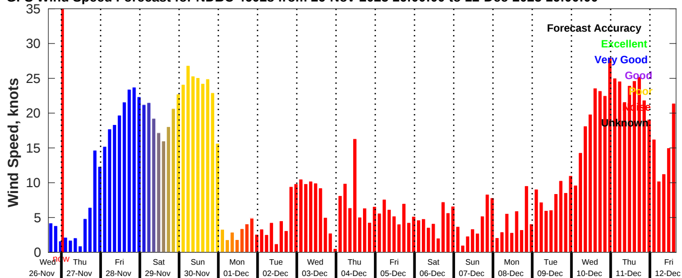
GFS Wind Speed Forecast for NDBC 46028 from 26-Nov-2025 16:00:00 to 12-Dec-2025 16:00:00
