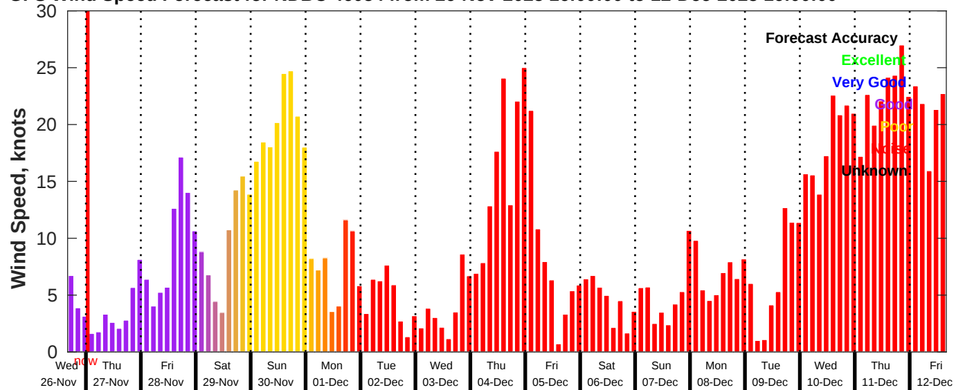
GFS Wind Speed Forecast for NDBC 46054 from 26-Nov-2025 16:00:00 to 12-Dec-2025 16:00:00
