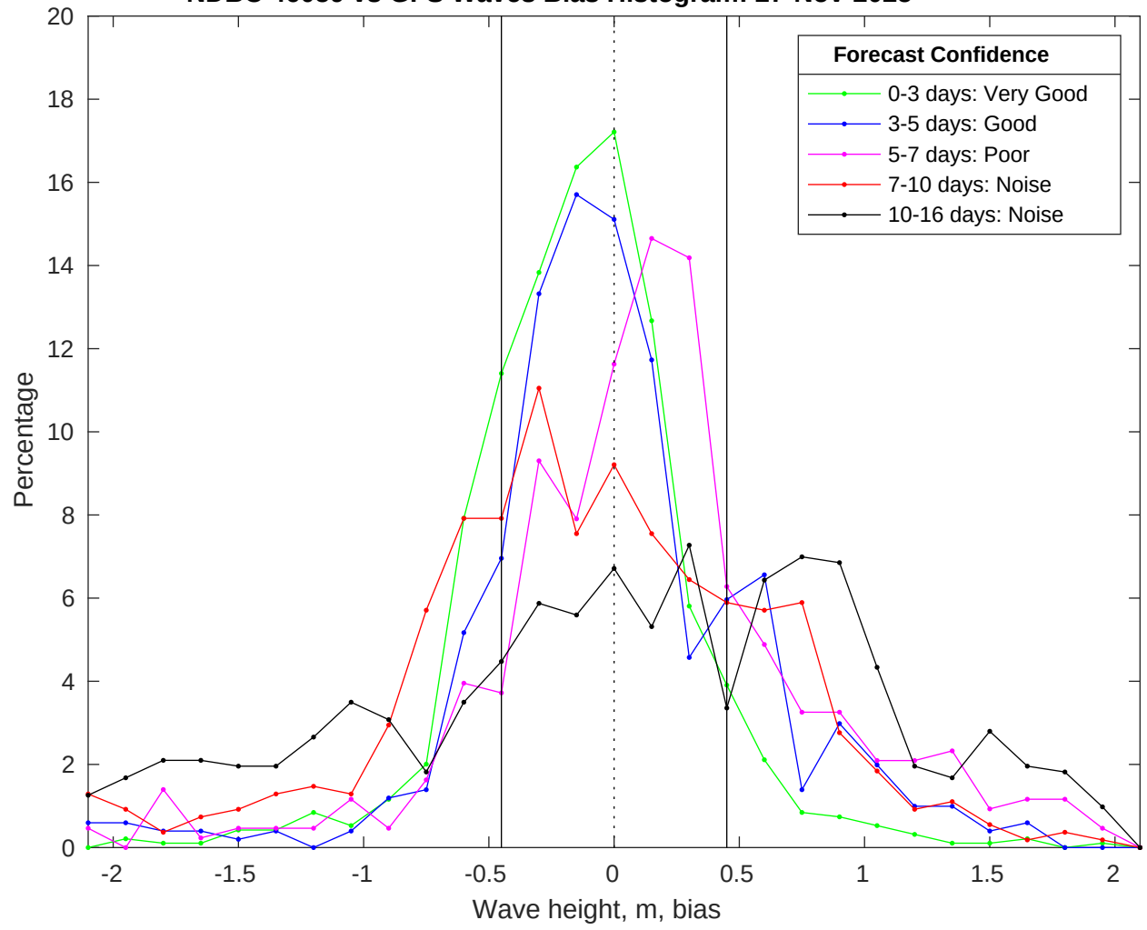
NDBC 46059 vs GFS Waves Bias Histogram: 27-Nov-2025
