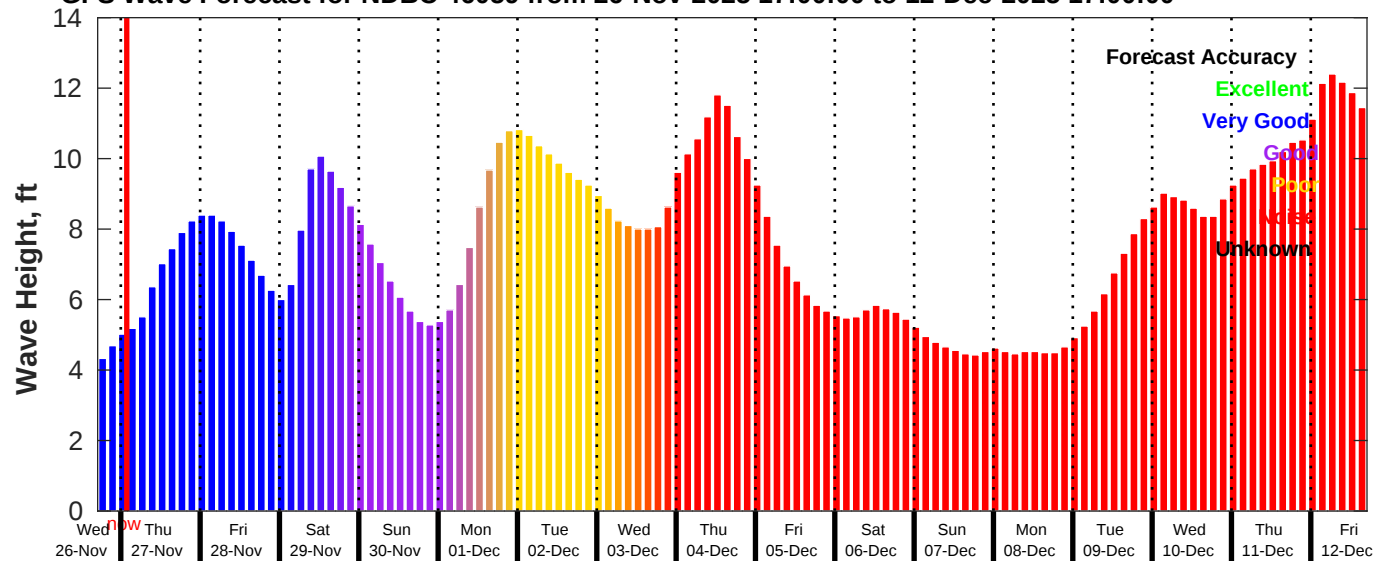
GFS Wave Forecast for NDBC 46059 from 26-Nov-2025 17:00:00 to 12-Dec-2025 17:00:00
