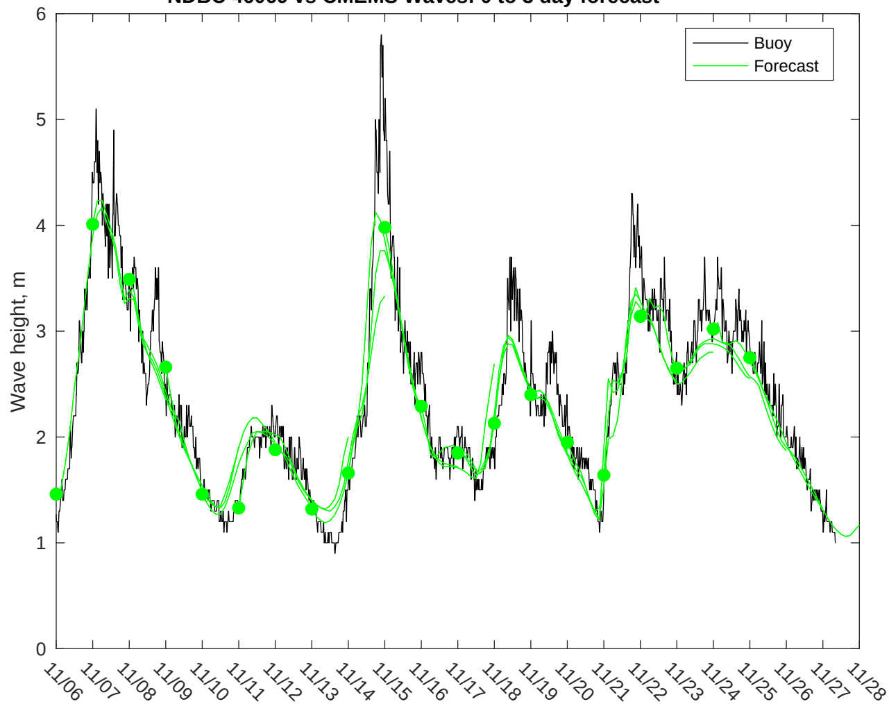
NDBC 46069 vs CMEMS Waves: 0 to 3 day forecast
