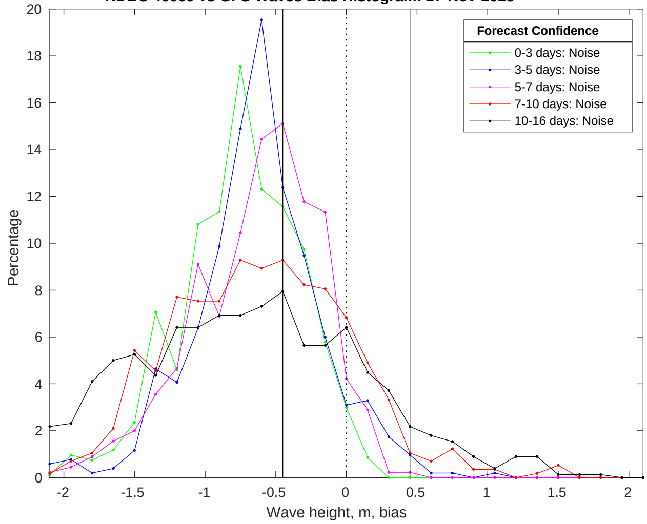
NDBC 46069 vs GFS Waves Bias Histogram: 27-Nov-2025
