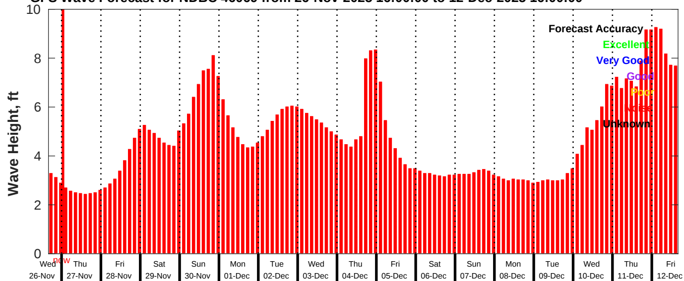
GFS Wave Forecast for NDBC 46069 from 26-Nov-2025 16:00:00 to 12-Dec-2025 16:00:00
