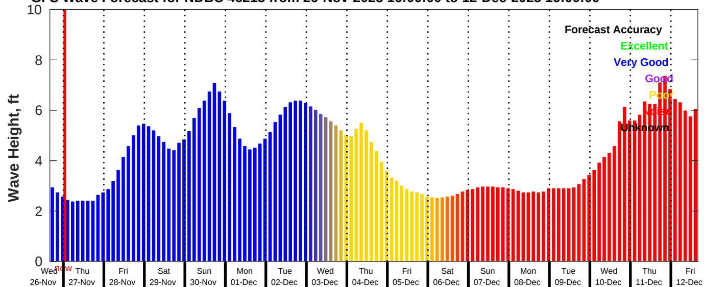
GFS Wave Forecast for NDBC 46215 from 26-Nov-2025 16:00:00 to 12-Dec-2025 16:00:00
