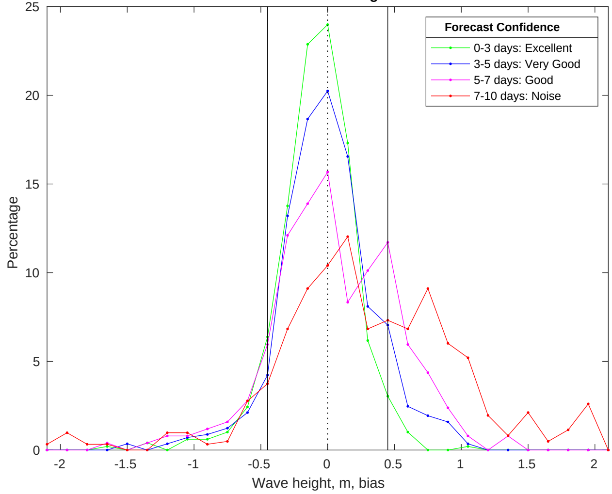
NDBC 46259 vs CMEMS Waves Bias Histogram: 27-Nov-2025
