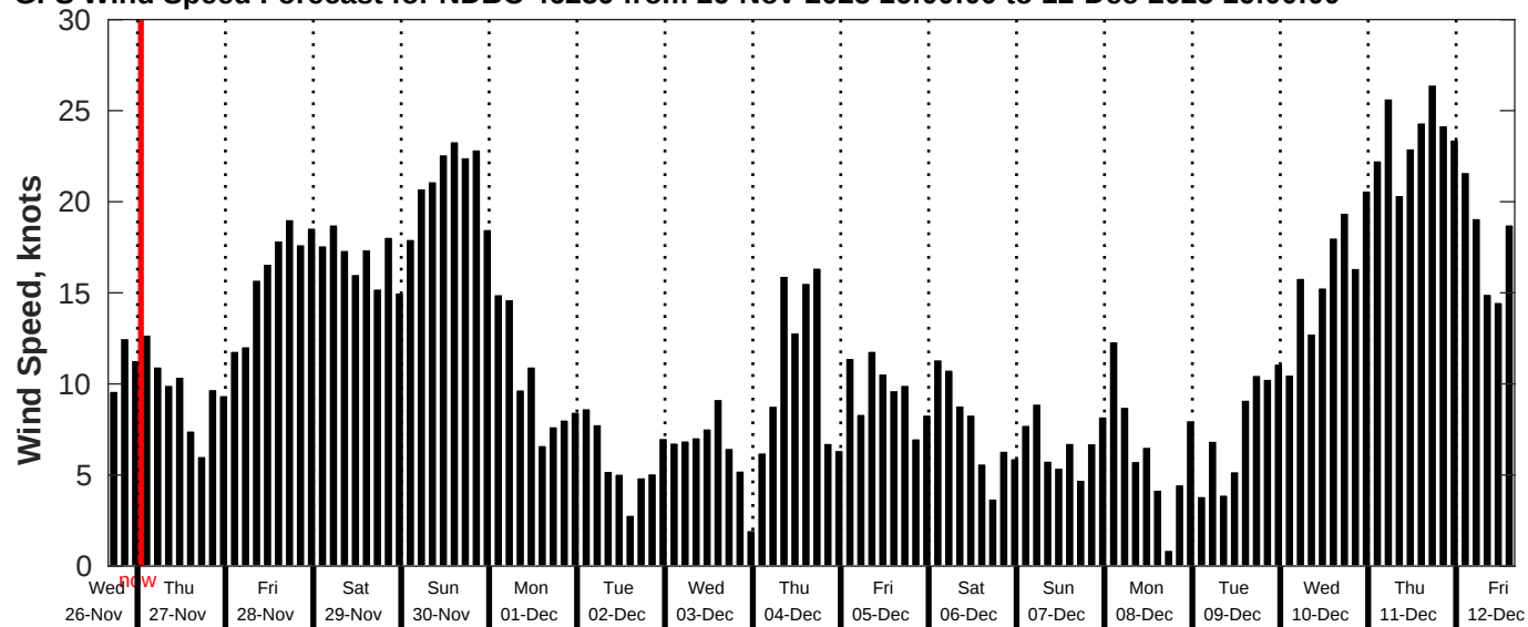
GFS Wind Speed Forecast for NDBC 46259 from 26-Nov-2025 16:00:00 to 12-Dec-2025 16:00:00
