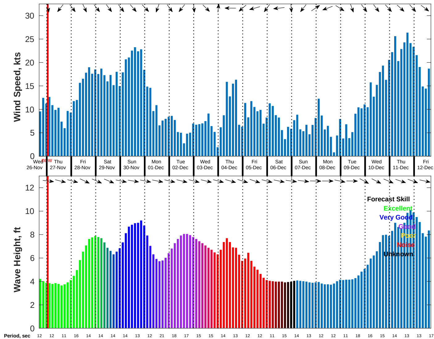
Wind & Wave Forecast for NDBC 46259 from 26-Nov-2025 16:00:00 to 12-Dec-2025 16:00:00
