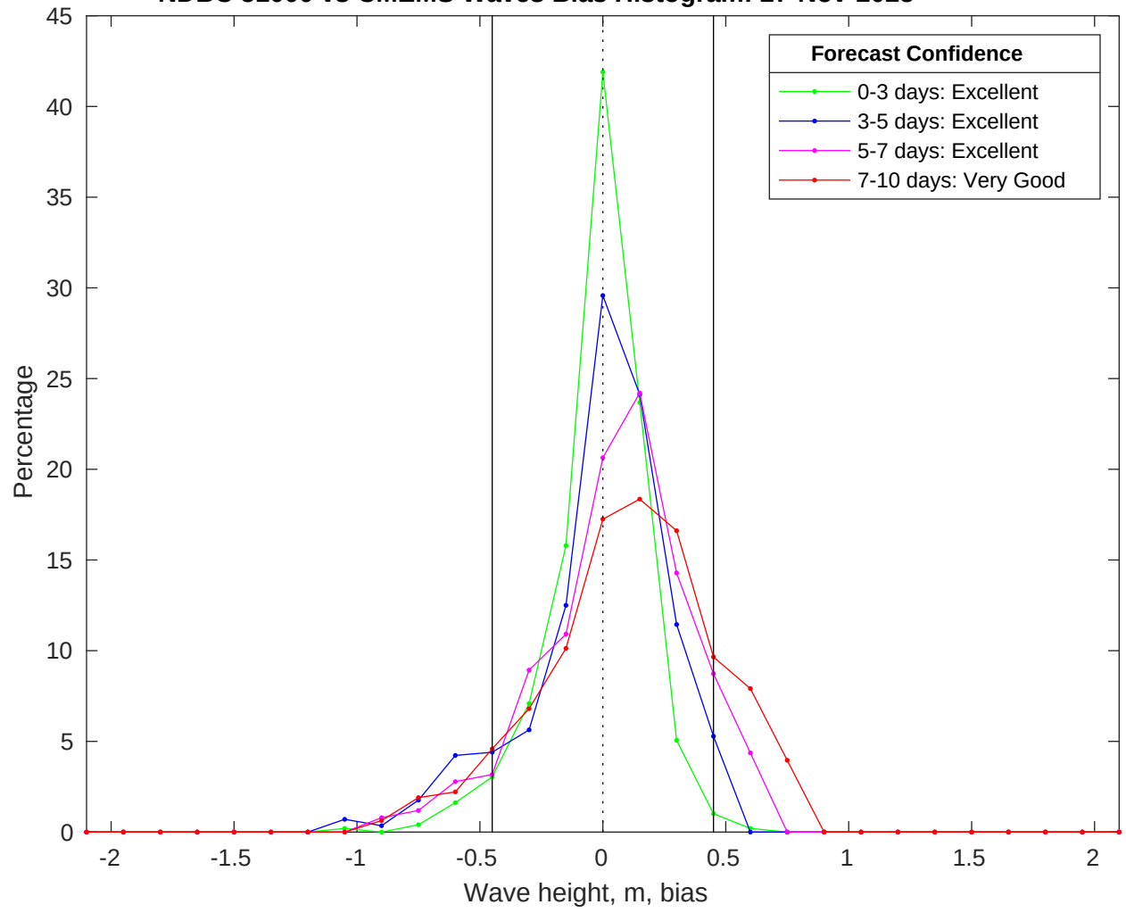
NDBC 51000 vs CMEMS Waves Bias Histogram: 27-Nov-2025
