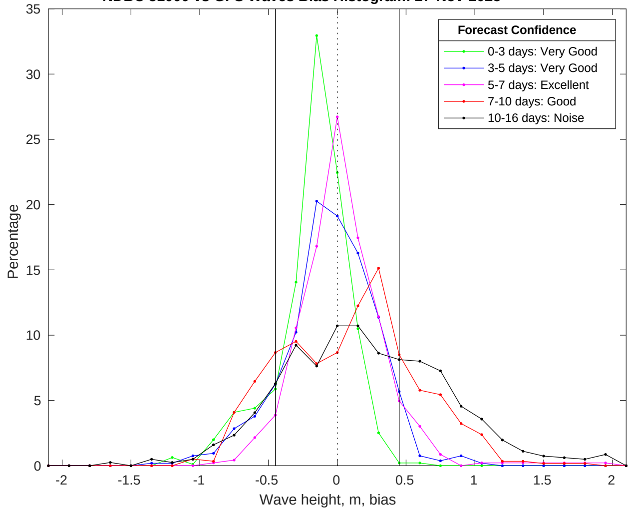
NDBC 51000 vs GFS Waves Bias Histogram: 27-Nov-2025
