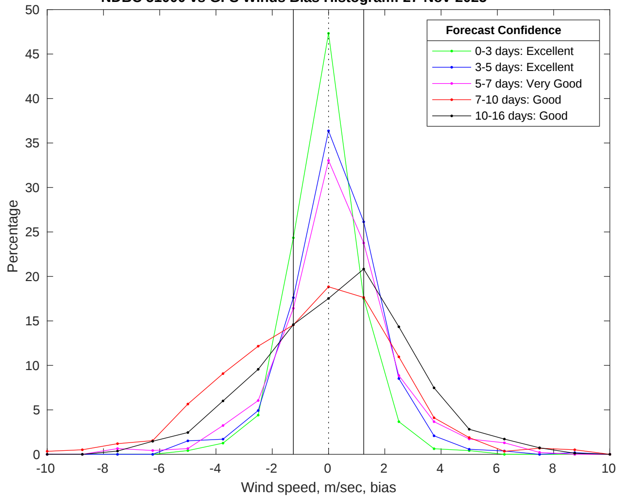
NDBC 51000 vs GFS Winds Bias Histogram: 27-Nov-2025
