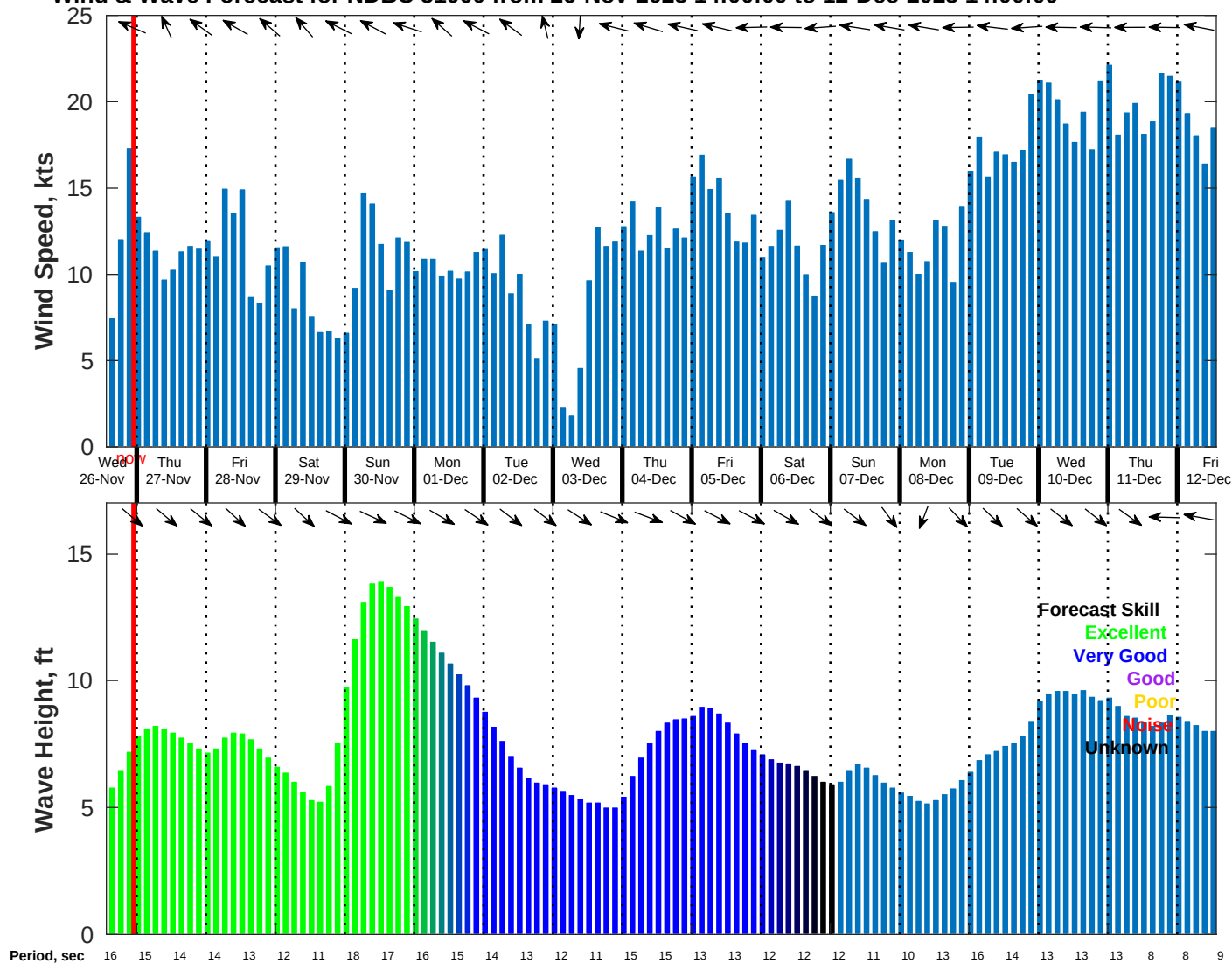
Wind & Wave Forecast for NDBC 51000 from 26-Nov-2025 14:00:00 to 12-Dec-2025 14:00:00
