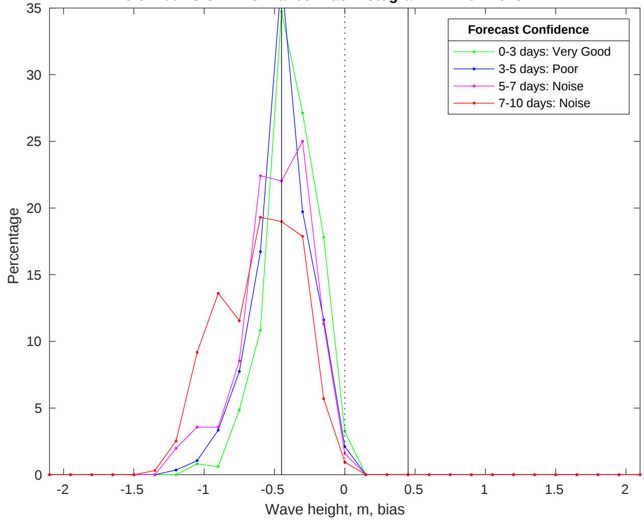
NDBC 51209 vs CMEMS Waves Bias Histogram: 27-Nov-2025
