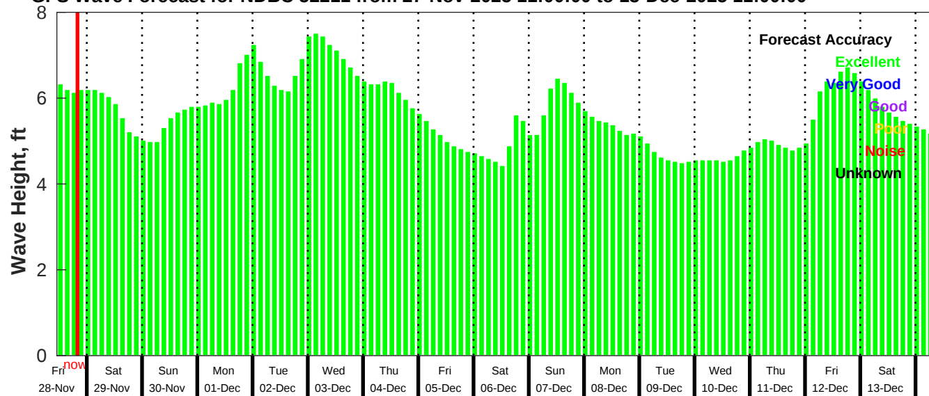
GFS Wave Forecast for NDBC 52211 from 27-Nov-2025 11:00:00 to 13-Dec-2025 11:00:00
