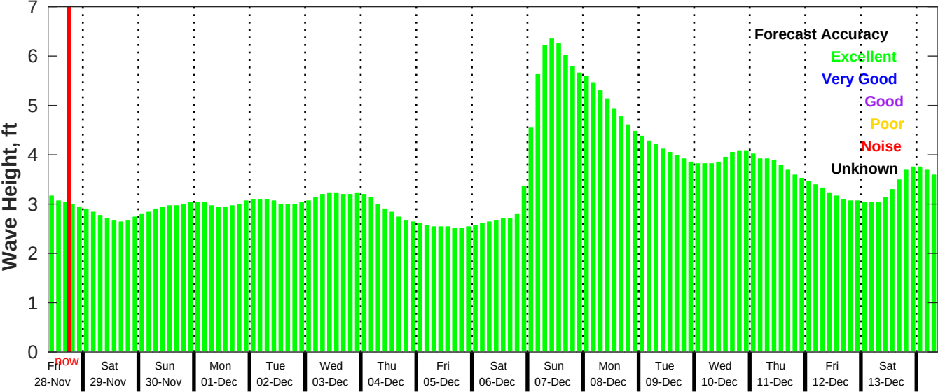
GFS Wave Forecast for NDBC 52212 from 27-Nov-2025 09:00:00 to 13-Dec-2025 09:00:00
