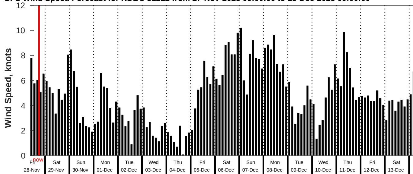
GFS Wind Speed Forecast for NDBC 52212 from 27-Nov-2025 09:00:00 to 13-Dec-2025 09:00:00
