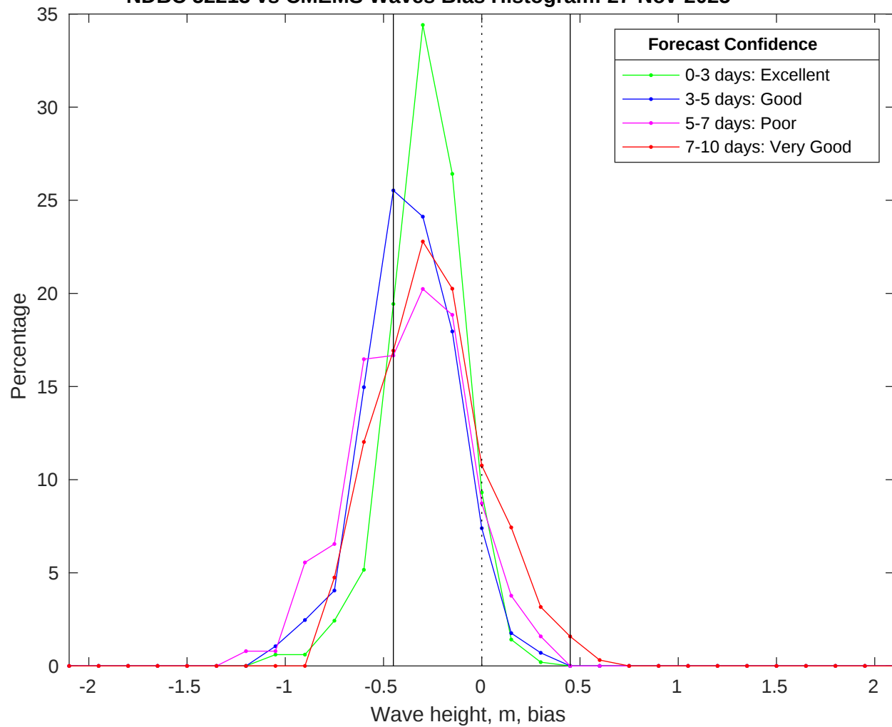
NDBC 52213 vs CMEMS Waves Bias Histogram: 27-Nov-2025
