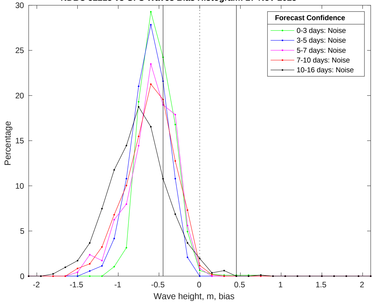
NDBC 52213 vs GFS Waves Bias Histogram: 27-Nov-2025
