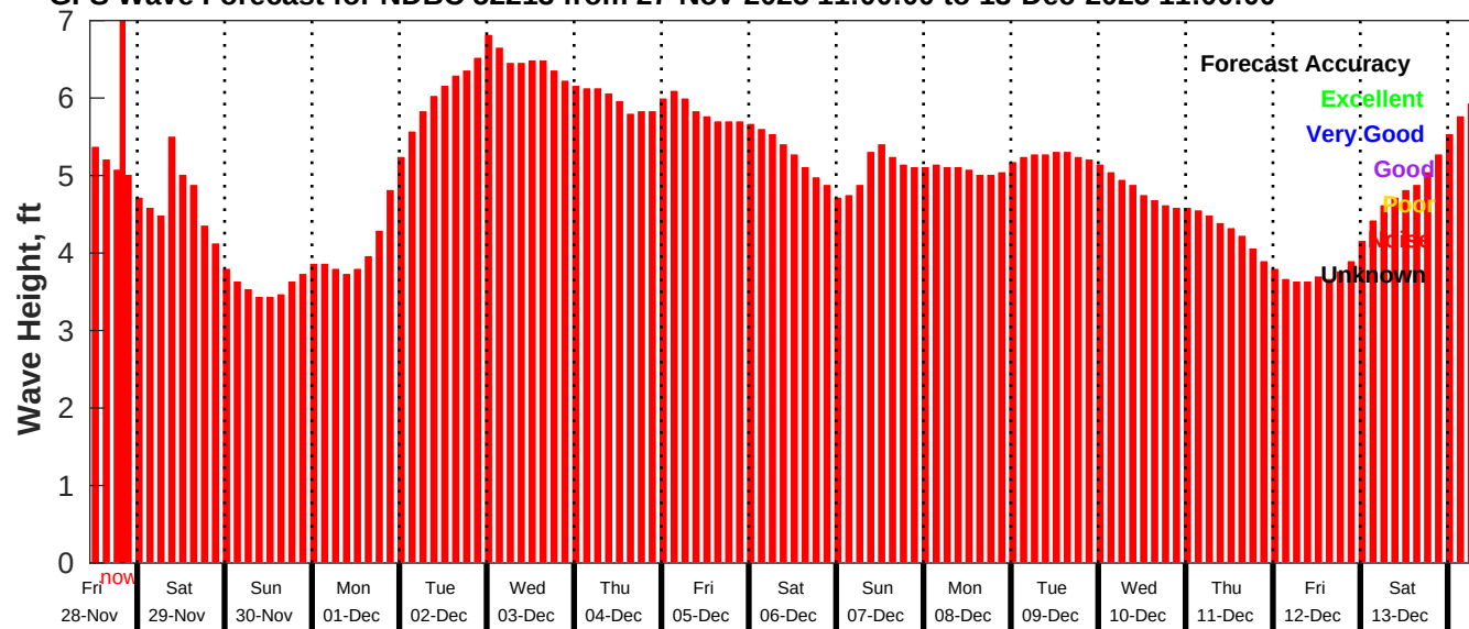
GFS Wave Forecast for NDBC 52213 from 27-Nov-2025 11:00:00 to 13-Dec-2025 11:00:00
