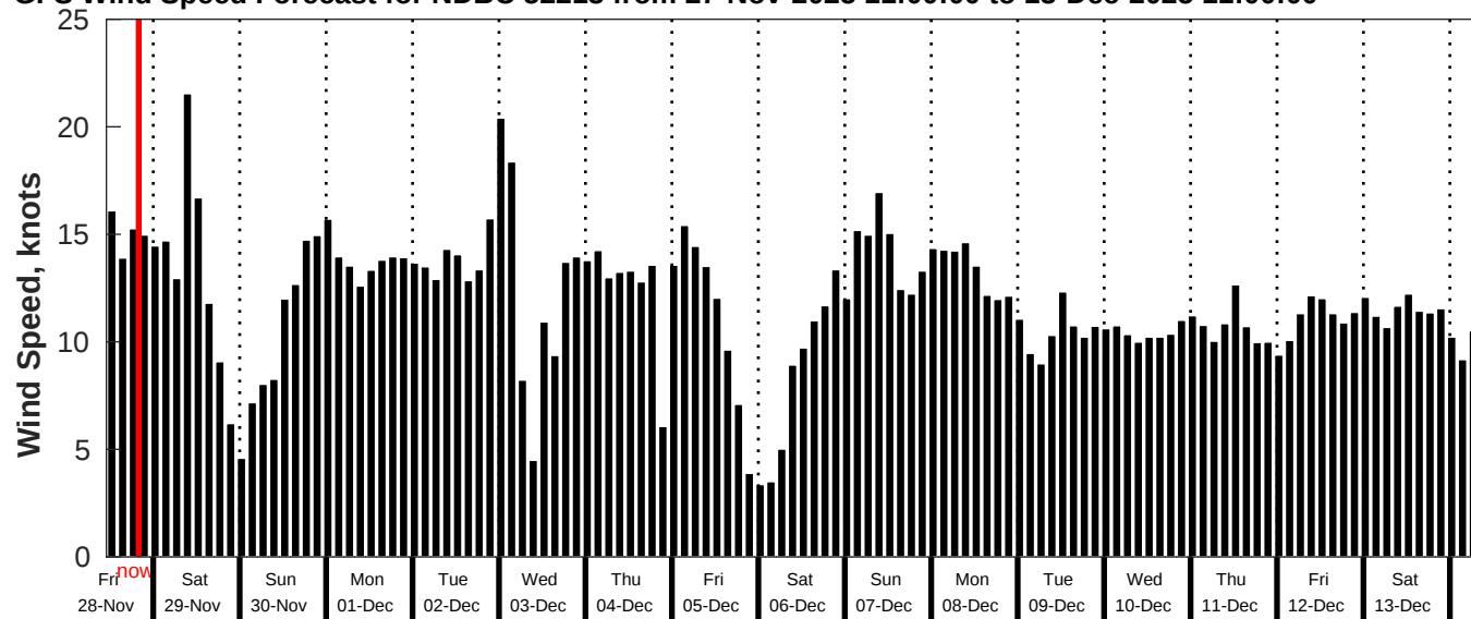
GFS Wind Speed Forecast for NDBC 52213 from 27-Nov-2025 11:00:00 to 13-Dec-2025 11:00:00
