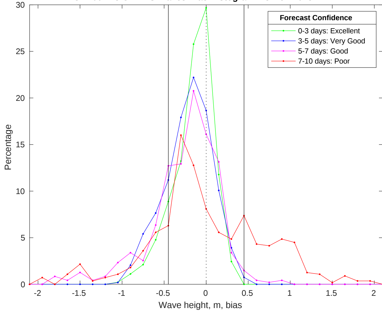
NDBC 41004 vs CMEMS Waves Bias Histogram: 28-Nov-2025
