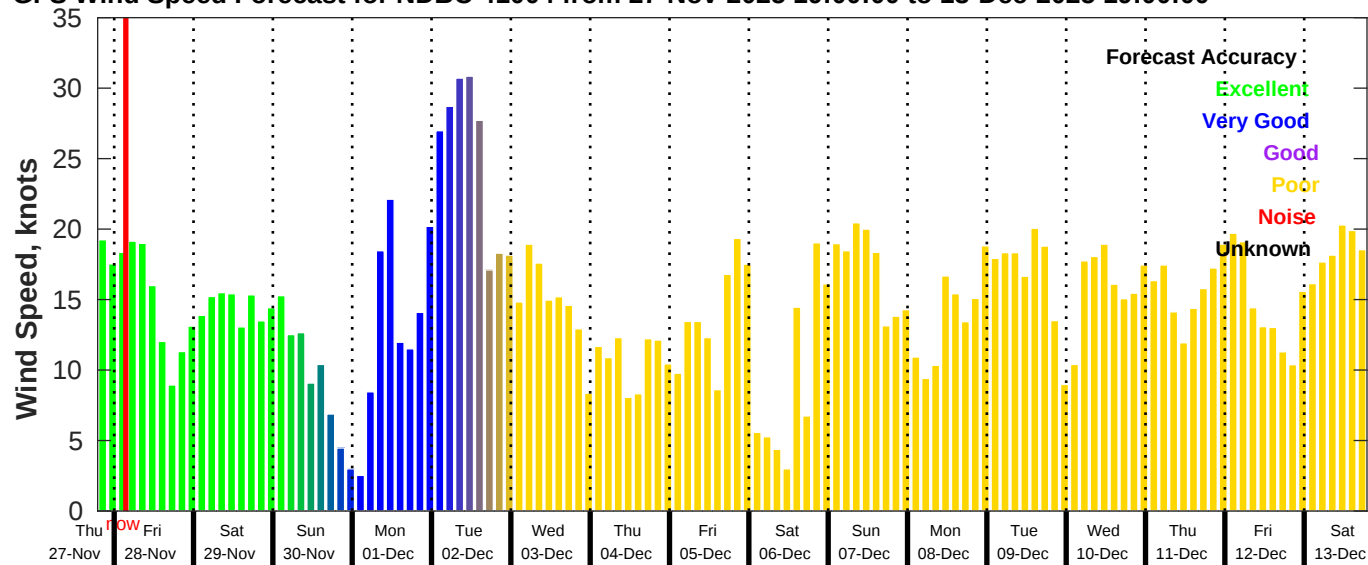
GFS Wind Speed Forecast for NDBC 41004 from 27-Nov-2025 19:00:00 to 13-Dec-2025 19:00:00
