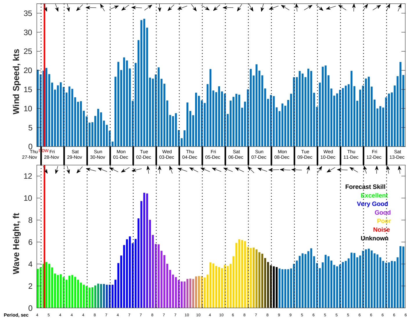
Wind & Wave Forecast for NDBC 41013 from 27-Nov-2025 19:00:00 to 13-Dec-2025 19:00:00
