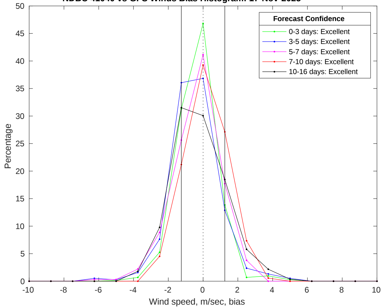
NDBC 41040 vs GFS Winds Bias Histogram: 17-Nov-2025
