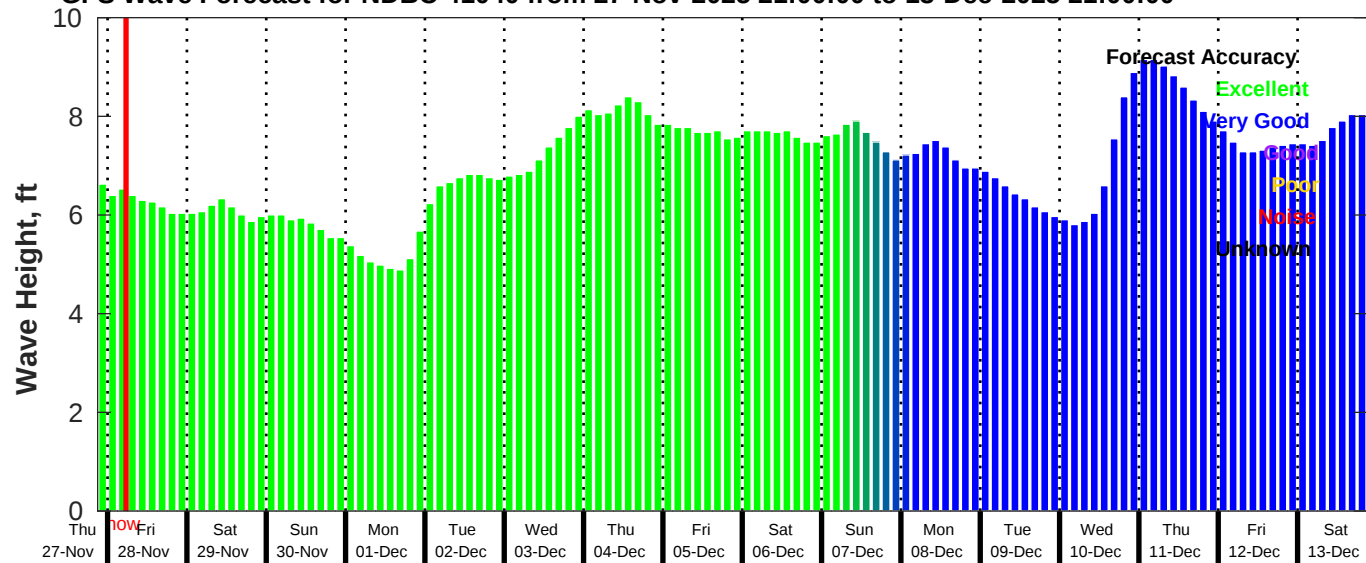
GFS Wave Forecast for NDBC 41040 from 27-Nov-2025 21:00:00 to 13-Dec-2025 21:00:00
